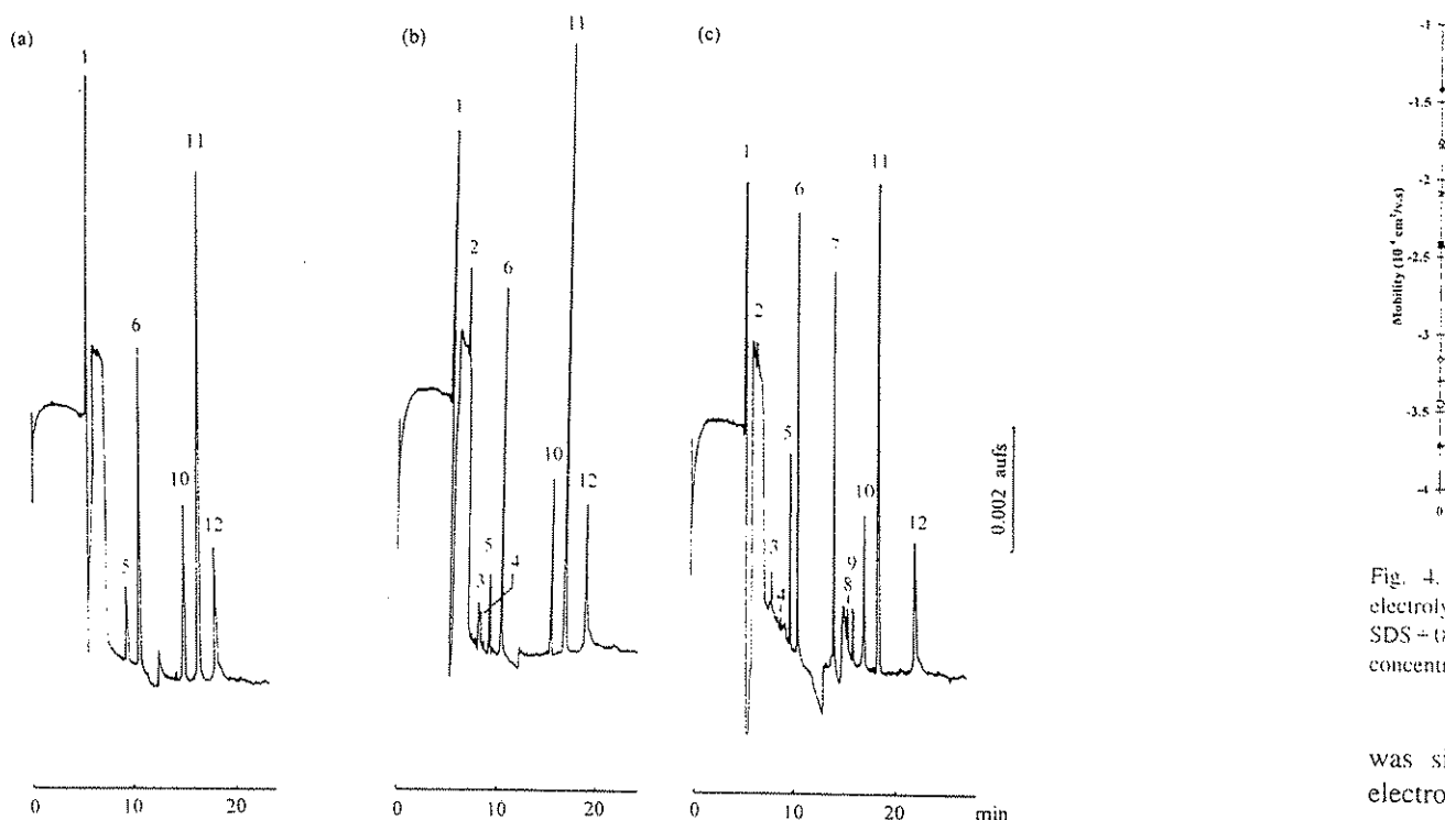
Fig. 3. Difference for resolution and detection among derivatization methods. Running electrolyte: 40 mM pH 7.0 \text{NaH}_2\text{PO}_4 - \text{Na}_2\text{B}_2\text{O}_7 buffer + 40 mM SDS-NTA (a and b; 0 mM; c: 7.5 mM). Sample mixture: 40 mM pH 6.0 \text{NaH}_2\text{PO}_4 - \text{Na}_2\text{B}_2\text{O}_7 buffer + NTA (a and c: 0 mM; b: 7.5 mM). Peaks (concentration): 1 = MeOH; 2 = DPLC (63.75 \mu\text{g}/\text{ml} ); 3 = Hg(II) (22.1 \mu\text{g}/\text{ml} ); 4 = Pb(II) (17.9 \mu\text{g}/\text{ml} ); 5 = PSC (66.25 \mu\text{g}/\text{ml} ); 6 = TMLC (63.5 \mu\text{g}/\text{ml} ); 7 = PMA (65 \mu\text{g}/\text{ml} ); 8 and 9 = Hg(I) (39.7 \mu\text{g}/\text{ml} ); 10 = Se (IV) (15 \mu\text{g}/\text{ml} ); 11 = TELC (68 \mu\text{g}/\text{ml} ); 12 = DPS (55 \mu\text{g}/\text{ml} ); 13 = NTA. Other conditions as in Fig. 1.
