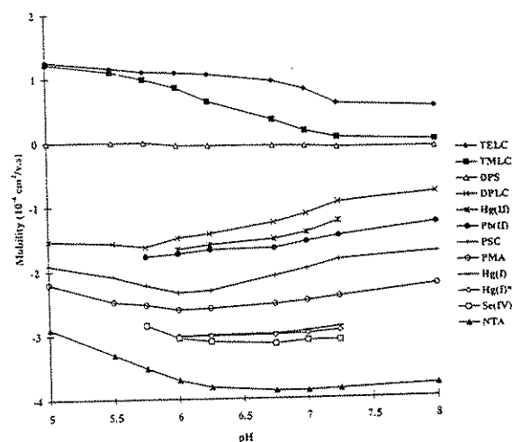
Fig. 1. Effect of pH on mobility. Running electrolyte: 40 mM pH 5.0–8.0 \text{NaH}_2\text{PO}_4\text{-Na}_2\text{B}_4\text{O}_7 buffer + 1.0 mM NTA; column: fused-silica capillary (63 cm \times 50 \mu\text{m} I.D.) with 50 cm length for separation; injection: 50 mbar \times 0.1 min; voltage: 20 kV; detection: 200 nm. Sample mixture: 40 mM pH 5.5 \text{NaH}_2\text{PO}_4\text{-Na}_2\text{B}_4\text{O}_7 buffer + 1.0 mM NTA + analytes.
