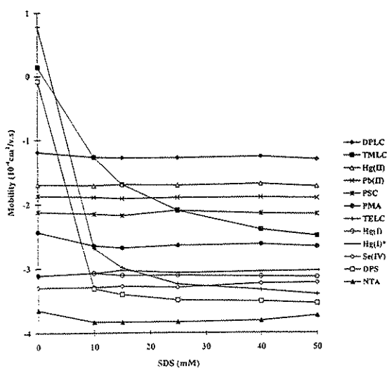
Fig. 2. Effect of SDS on mobility. Running electrolyte: 40 mM pH 7.0 \text{NaH}_2\text{PO}_4 - \text{Na}_2\text{B}_2\text{O}_7 buffer + 1.0 mM NTA -0–50 mM SDS. Other conditions as in Fig. 1, except pH 7.0 in sample mixture.
