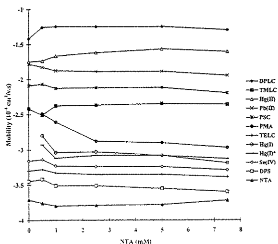
Fig. 4. Effect of NTA in the running electrolyte. Running electrolyte: 40 mM pH 7.0 \text{NaH}_2\text{PO}_4 - \text{Na}_2\text{B}_2\text{O}_7 buffer + 40 mM SDS + 0–7.5 mM NTA. Other conditions as in Fig. 3 except NTA concentration 2.5 mM in the sample mixture.
