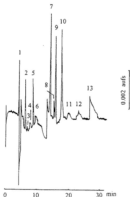
Fig. 6. Electropherogram generated using AFSI, 50 mbar \times 0.15 min for water plug; +20 kV 2.0 min and -20 kV 1.90 min for sample stacking. Concentrations of the sample matrix and all solutes were 1/40 and 1/200, respectively, as for Fig. 5. Other conditions as in Fig. 5.
